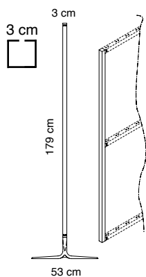
5203/BP-GA, 5203/BP-BO 1-way up-right
