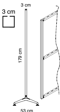
5203/B-GA, 5203/B-BO 1-way up-right
